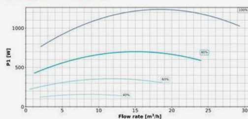
POWER CONSUMPTION 1.5 HP
