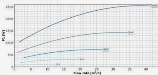
POWER CONSUMPTION 3 HP
